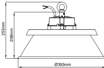
Universal Reflector
