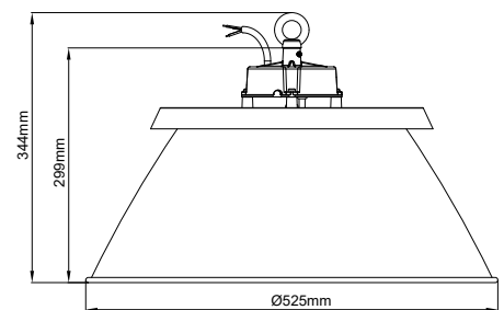
Tall Reflector
