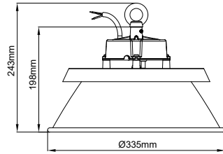
Universal Reflector
